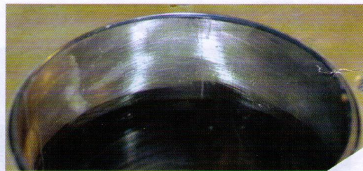
Honing grooves are critical for holding oil on the cylinder. Use the wrong oil during break-in and you risk glazing over these grooves
