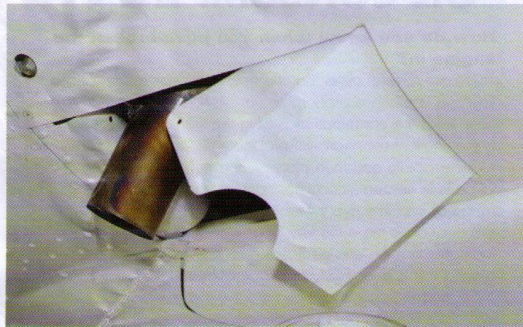
Be generous with cooling air during break-in. Also monitor the inside colour of the exhaust stub to help judge the progress of break-in
